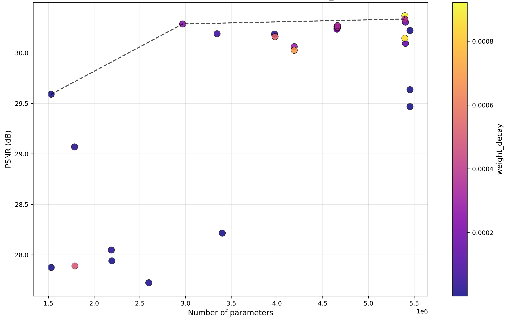
PSNR vs #Params — WaveletAttention — by weight_decay
